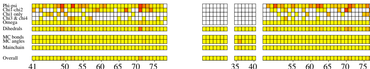
g. G-factors
